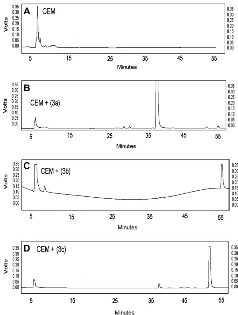
Fig. 4. HPLC-UV chromatograms of untreated CEM cells (A), CEM cells treated with (3a) (B), CEM cells treated with (3b) (C), and CEM cells treated with (3c) (D).
