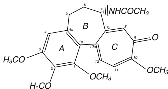
Fig. 1. Structure of colchicine.
