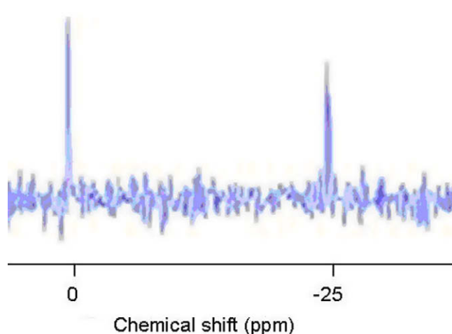
Fig. 6. ^{19}\text{F} MRS of CEM cells treated with ( 5c ). \text{CF}_3\text{COOH} was used as chemical shift reference at 0 ppm.
