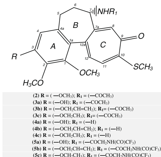
Fig. 2. Derivatives of thicolchicine.
