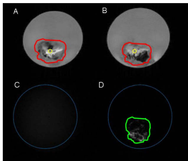
Fig. 5. An MR images of the CEM cells in the hollow fiber bioreactor at 9.4 T. The solid red line indicates the area of cells and yellow solid line indicated the fiber. The images: ^1\text{H} MRI of cells before treatment with ( 5c ) (A) and after 72 h treatment with ( 5c ) derivative (B). Spin echo (SE) pulse sequence (TR/TE = 5000/12.8 ms, FOV = 3 cm \times 3 cm, slice thickness 1 mm and matrix 256 \times 256) was used. ^{19}\text{F} MRI of cells before treatment with ( 5c ) (C) and after 72 h treatment with ( 5c ) derivative (D). The blue line at ^{19}\text{F} images indicates contour of HFB device and the green solid line indicated treated cells. Inversion Recovery (IR) spin-echo method with Inversion Time (IT) equal to 400 ms and TE/TR = 16.5/5000 ms, slice thickness 1 mm and matrix 256 \times 256 was used.
