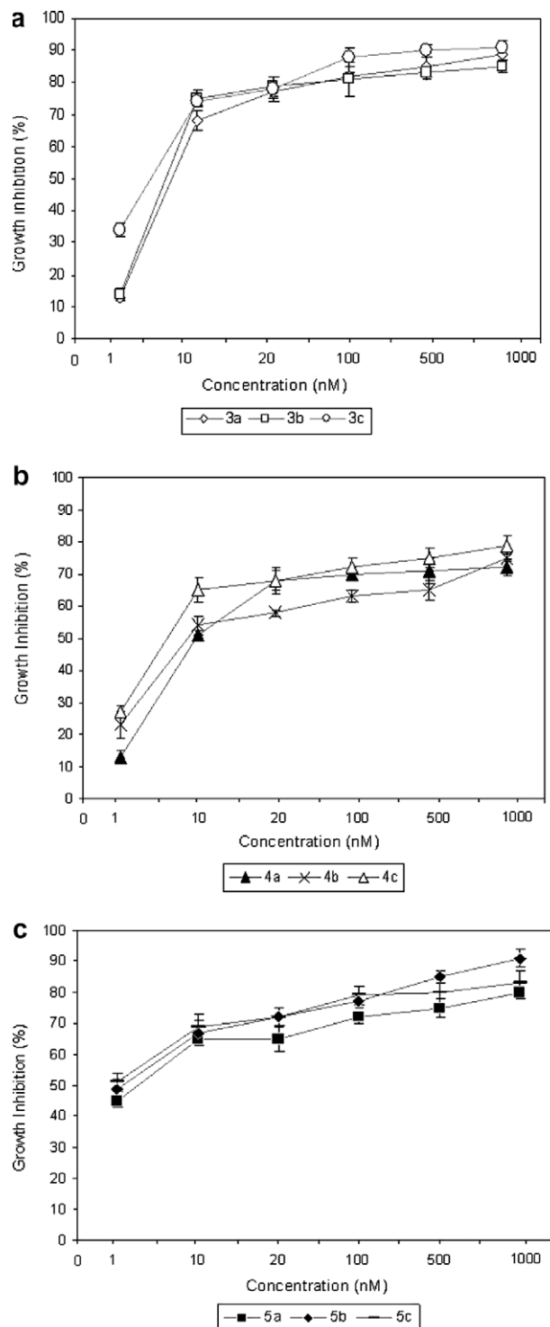
Fig. 3. Effects of various doses of derivatives on CEM cells. Data points indicated the inhibitory percentage of cells \pm SD in each treatment group: ( 3a–c ) (A), ( 4a–c ) (B) and ( 5a–c ) (C), as compared with controls.
